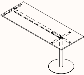
Wall Mounted Table Single Beam OH 750/1050mm* Base DIA 720mm
