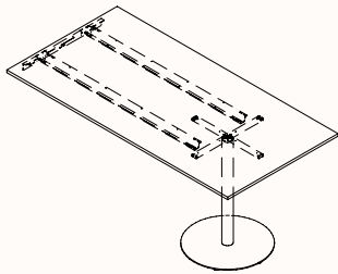
Wall Mounted Table Double Beam OH 750/1050mm* Base DIA 720mm
