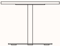
Coffee Table OH 425mm* Base DIA 580mm
